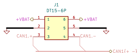
DT15-6P EXPANSION CONNECTOR
