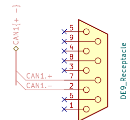
KVASER LEAF DEBUG CONNECTOR
