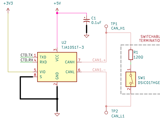
CAN TRANCEIVER
